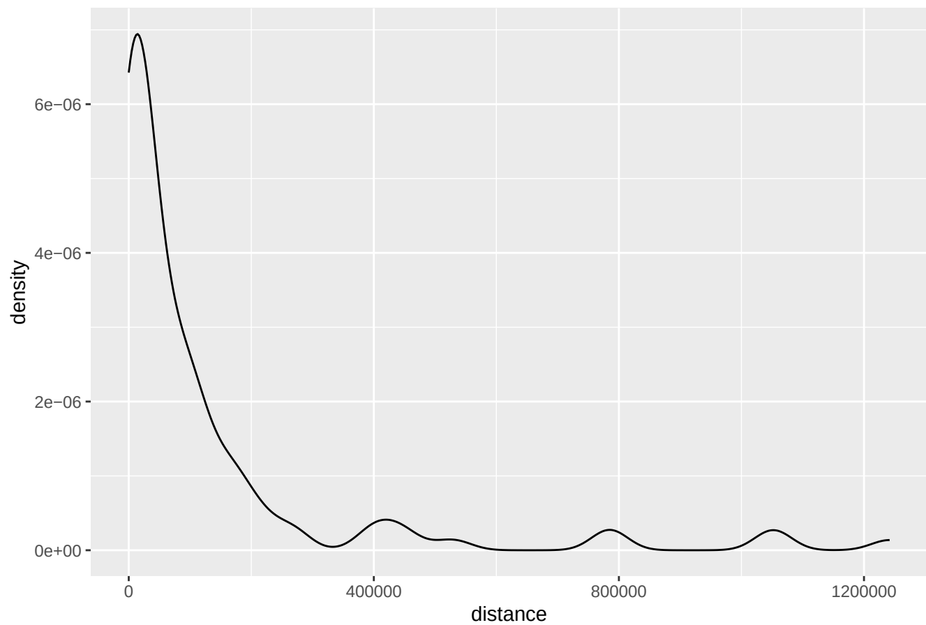
density of MER61E TEs distance to expressed gene
